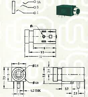
ST-003 (ø2.5mm Type)
