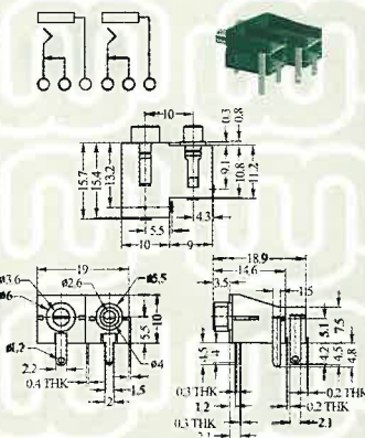
PY-6401N (ø3.5mm/2.5mm Type)
