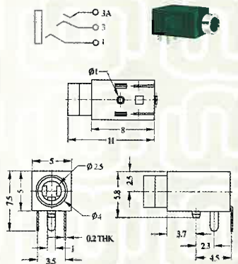
ST-002 (ø2.5mm Type)
