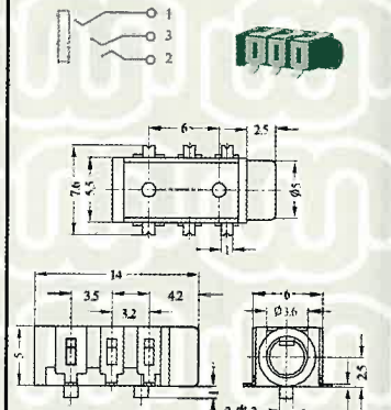
ST-019 (ø3.5mm Type)
