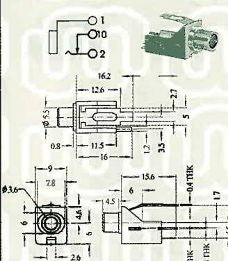
EY-503NR (ø3.5mm Type)
