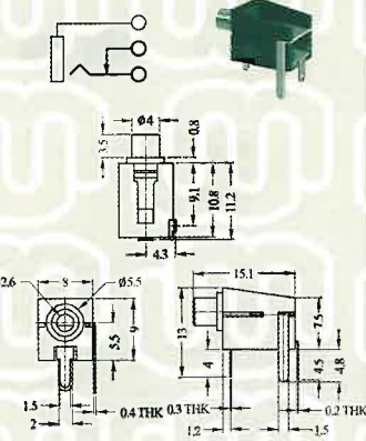
PY-401N (ø2.5mm Type)
