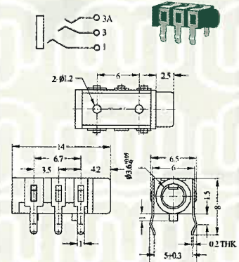
ST-009 (ø3.5mm Type)
