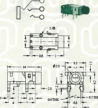
ST-007 (ø3.5mm Type)
