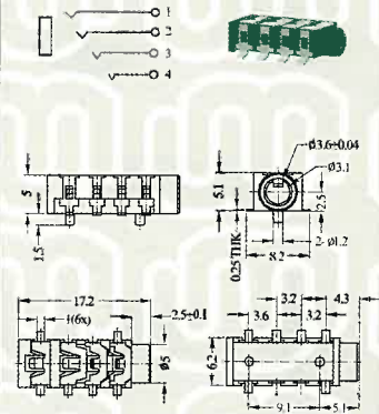
ST-012 (ø3.5mm Type)
